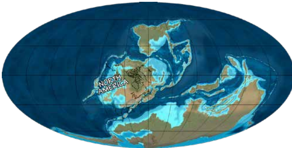
Figure 4.7: Earth during the late Devonian, about 370 million years ago.
