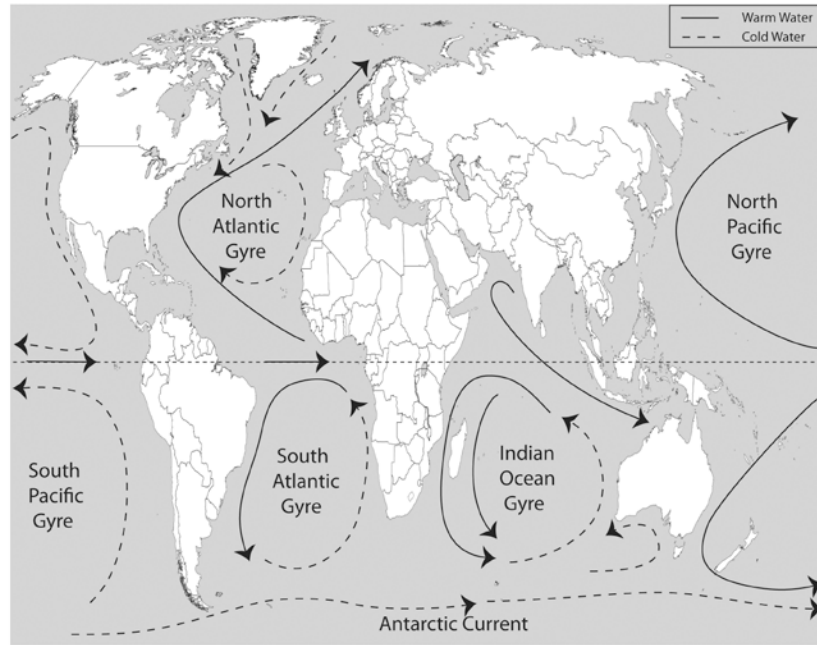
Ocean Circulation Patterns
