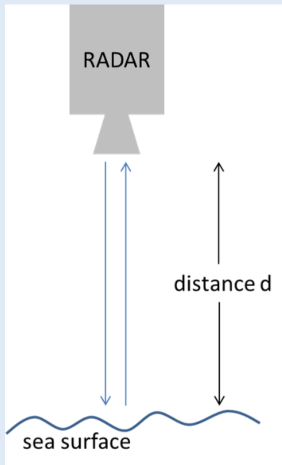
Schematic of a radar-based tide gauge.
