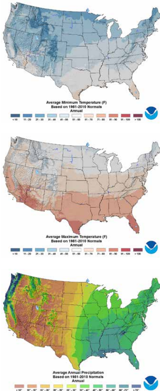
Figure 6.1: Maps of 1981-2010 climate normals (30-year averages for this time period) for the contiguous United States: A) annual minimum temperature (°F); B) annual maximum temperature (°F); and C) annual precipitation (inches). (See Teacher-Friendly Guide website for a full color version.)
