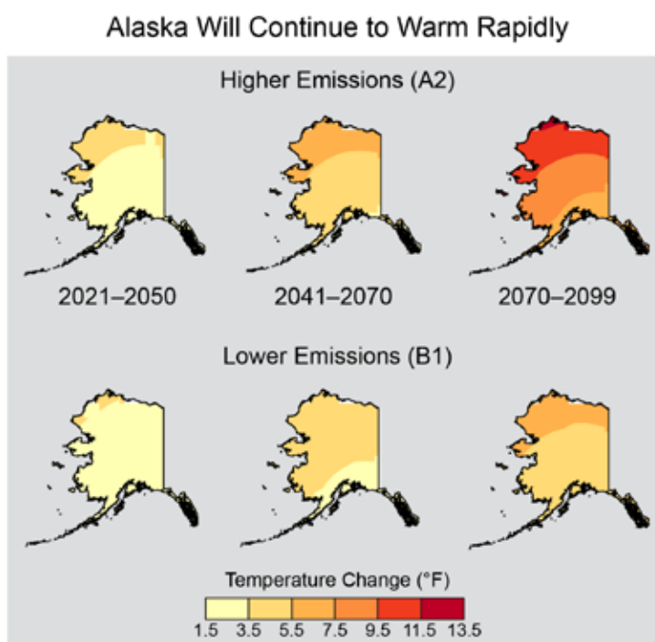
Figure 6.24: Northern latitudes are warming faster than more temperate regions, and Alaska has already warmed much faster than the rest of the country. Maps show changes in temperature, relative to 1971–1999, projected for Alaska in the early, middle, and late parts of this century, if heat-trapping gas (also known as greenhouse gas) emissions continue to increase (higher emissions, A2) or are substantially reduced (lower emissions, B1). (See Teacher-Friendly Guide website for a full color version.)
