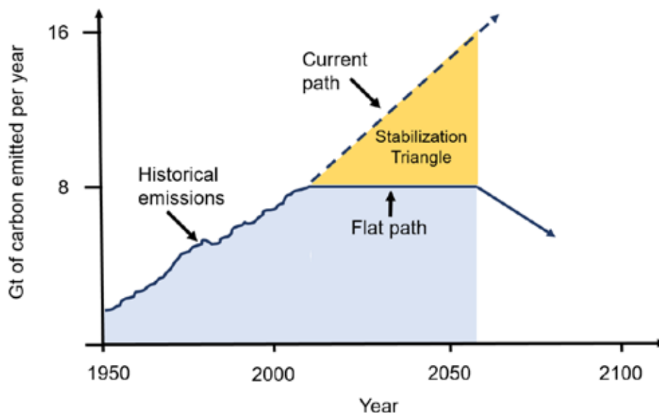
Figure 7.1: Carbon emissions over time, including historical emissions and two future paths, one following the current trend and one that remains flat and eventually decreases. The area between these paths is called the Stabilization Triangle, and represents the future emissions we will need to avoid to move from the current path to the flat path. (See Teacher-Friendly Guide website for a full color version.)
