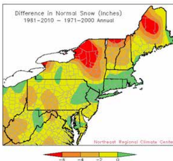
Figure 6.3: Difference between 30-year averages of snow depth for the Northeast. The comparison shows a decline in snow depth over much of the Northeast when comparing the years 1981-2010 and 1971-2000. (See Teacher-Friendly Guide website for a full color version.)
