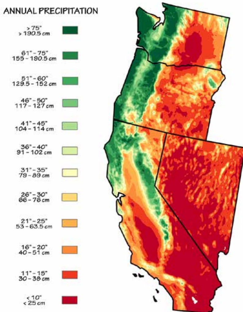
Figure 6.17: Mean annual precipitation for the West Coast. (See Teacher-Friendly Guide website for a full color version.)
